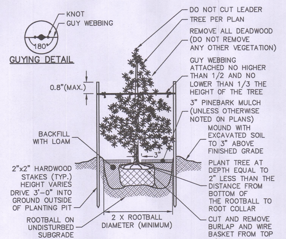
Evergreen Tree Planting Detail (4'-0" High and Greater) NOT TO SCALE
