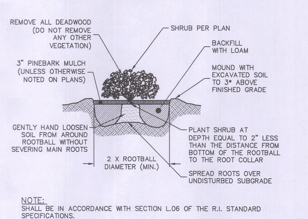
Container Grown Shrub Planting Detail NOT TO SCALE
