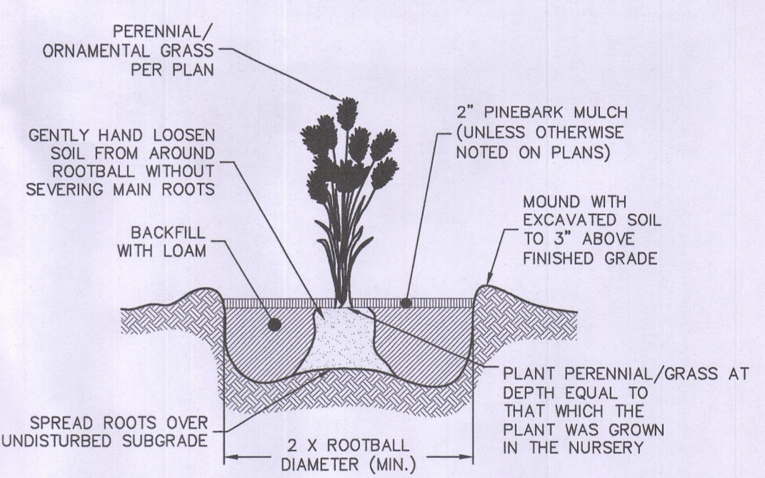
Perennial/Ornamental Grass Planting Detail NOT TO SCALE
