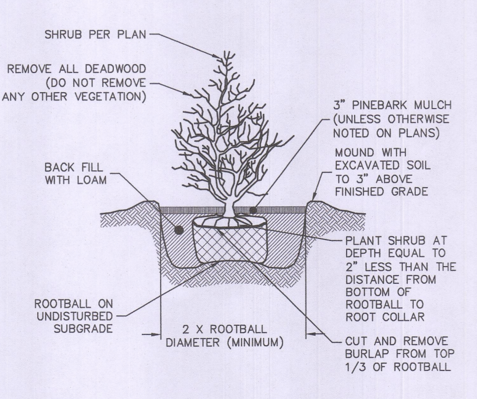
Ball and Burlap Shrub Planting Detail NOT TO SCALE
