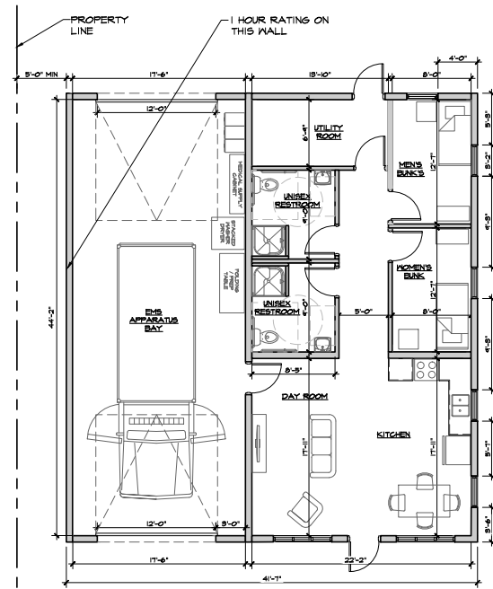
PROPOSED EMS STATION FLOOR PLAN
