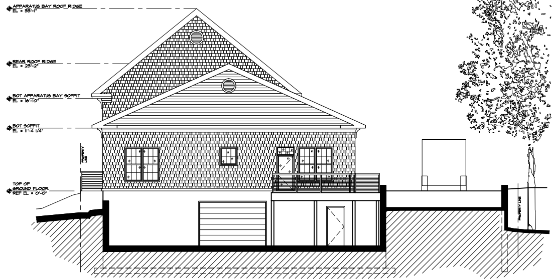
NORTH ELEVATION
