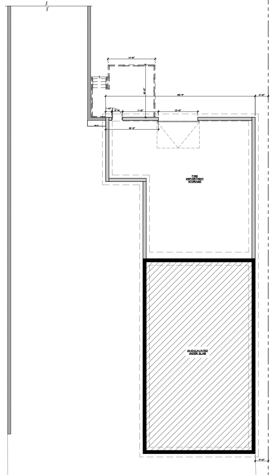
PROPOSED FIRE STATION BASEMENT PLAN
