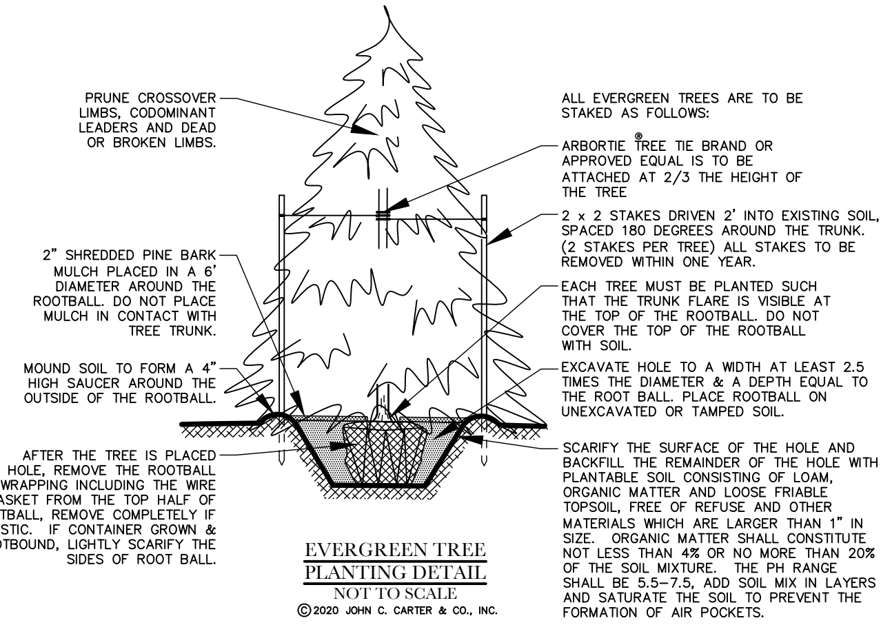
SHRUB PLANTING DETAIL NOT TO SCALE © 2020 JOHN C. CARTER & COMPANY, INC.
