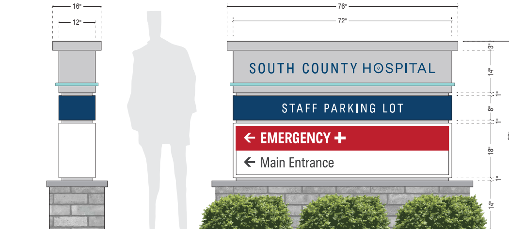
2 End View Fabrication Scale: 1:10
