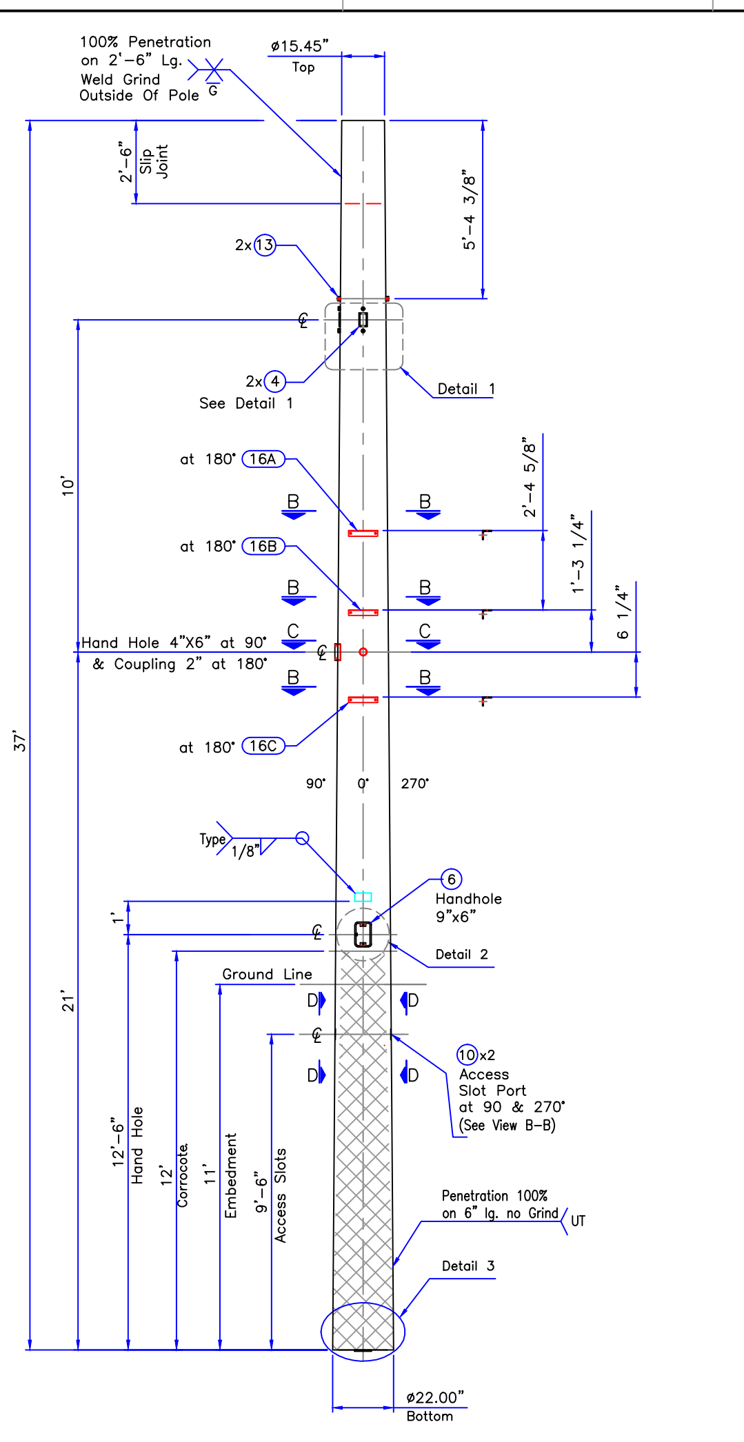
Bottom Section 3/16" Thk. ASTM A-572 GR 65
