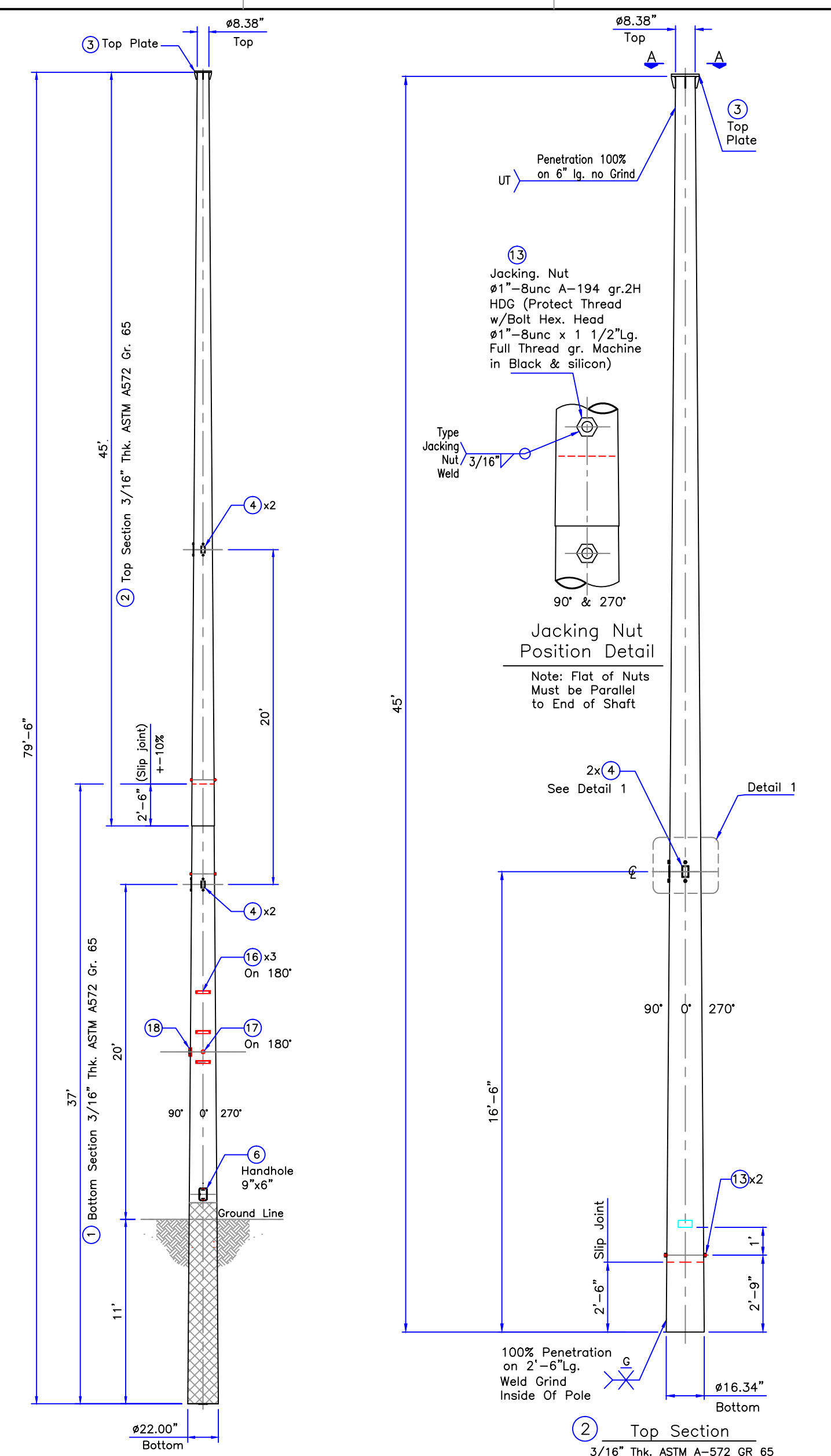
TSL75HA Pole Elevation Round Tapered Pole 2 Sections
